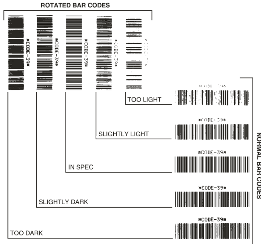
Figure 22 • Bar Code Darkness Comparison
