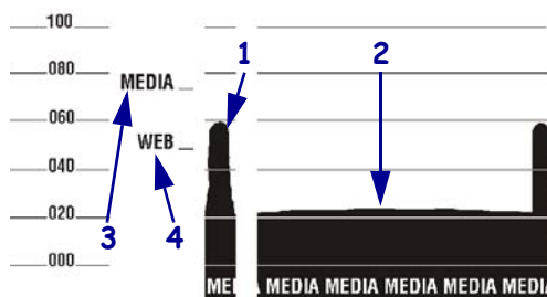
Figure 25 • Sensor Profile (Media Section)
