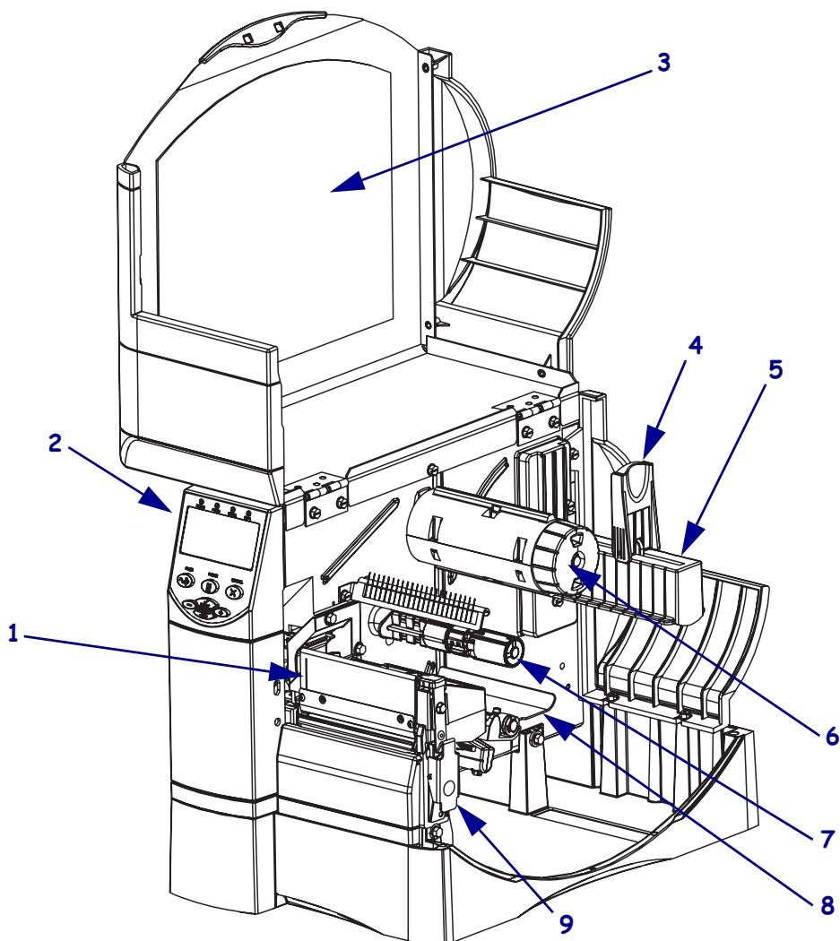
Figure 4 • Printer Components
