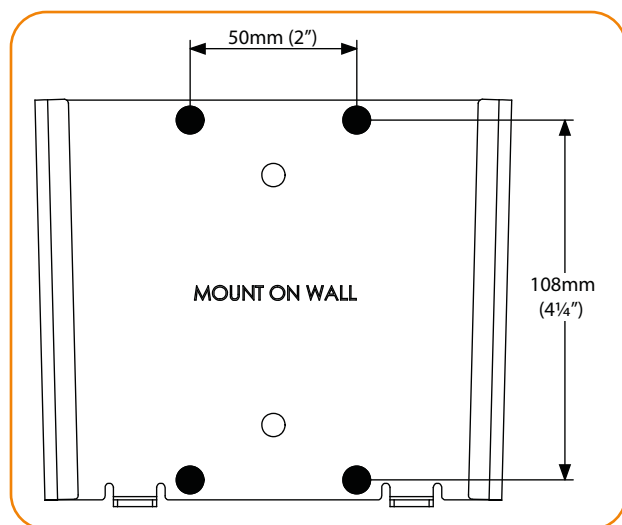
Mounting hole pattern for: Dry Wall
