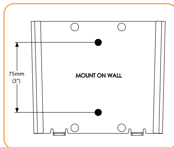
Mounting hole pattern for: Masonry Wall and Timber Stud
